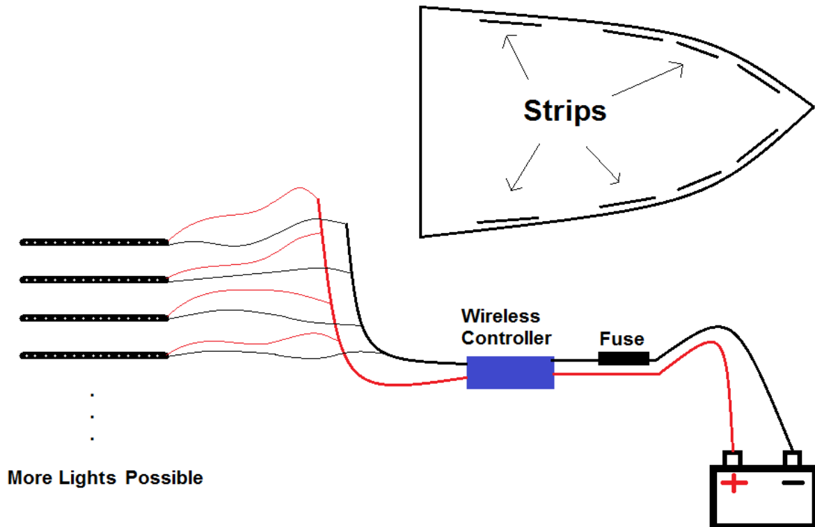
Figure 1. Wiring diagram and example strip placement
